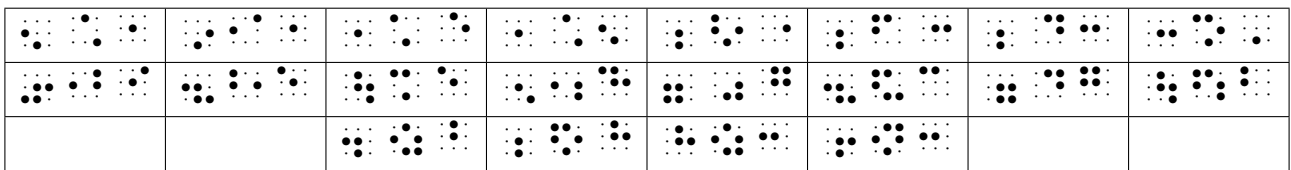
Models with group G_9 = \langle a, b, c \mid a^2, b^2, c^2, acbacbcabc \rangle
