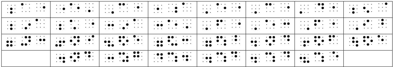
Models with group G_8 = \langle a, b, c \mid a^2, b^2, c^2, (ab)^3, (bc)^3 \rangle
